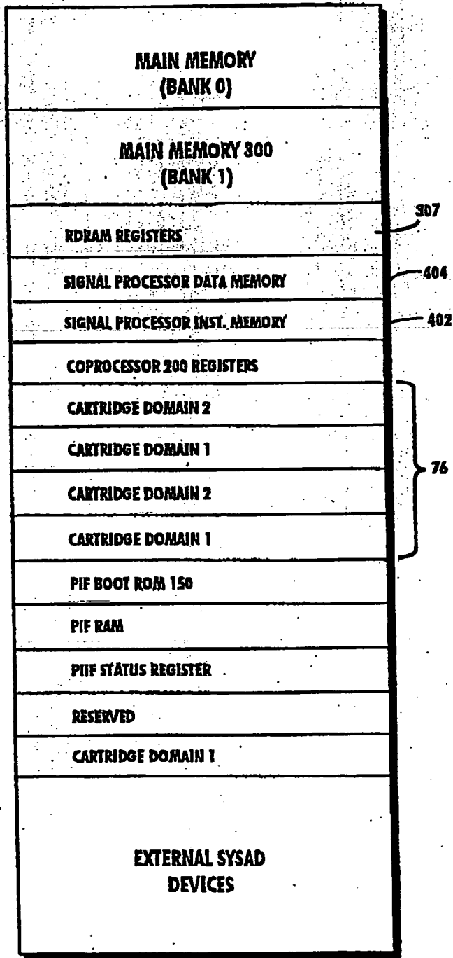
Fig. 5B EXAMPLE CPU MEMORY MAP
